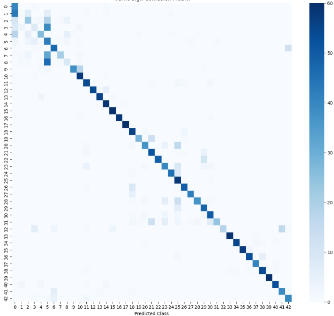
Traffic Sign Confusion Matrix
